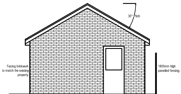
SIDE ELEVATION AS PROPOSED (1:50)
