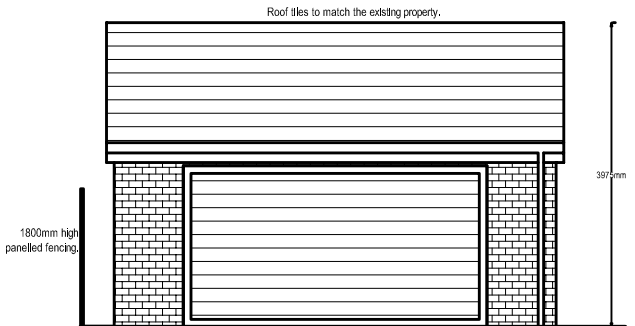
FRONT ELEVATION AS PROPOSED (1:50)
