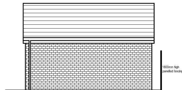
REAR ELEVATION AS PROPOSED (1:50)
